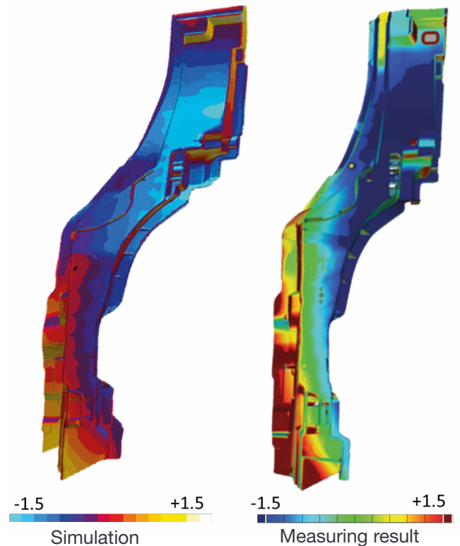
Evaluation of the predicted distortion using the 6-point method (simulation vs. measuring result)
