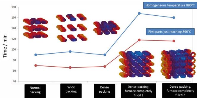
Austenitization times for different charges
