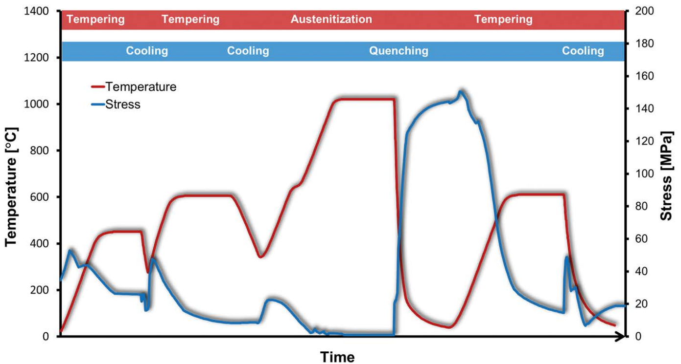
Characteristic temperature profile and associated stress evolution during heat treatment
